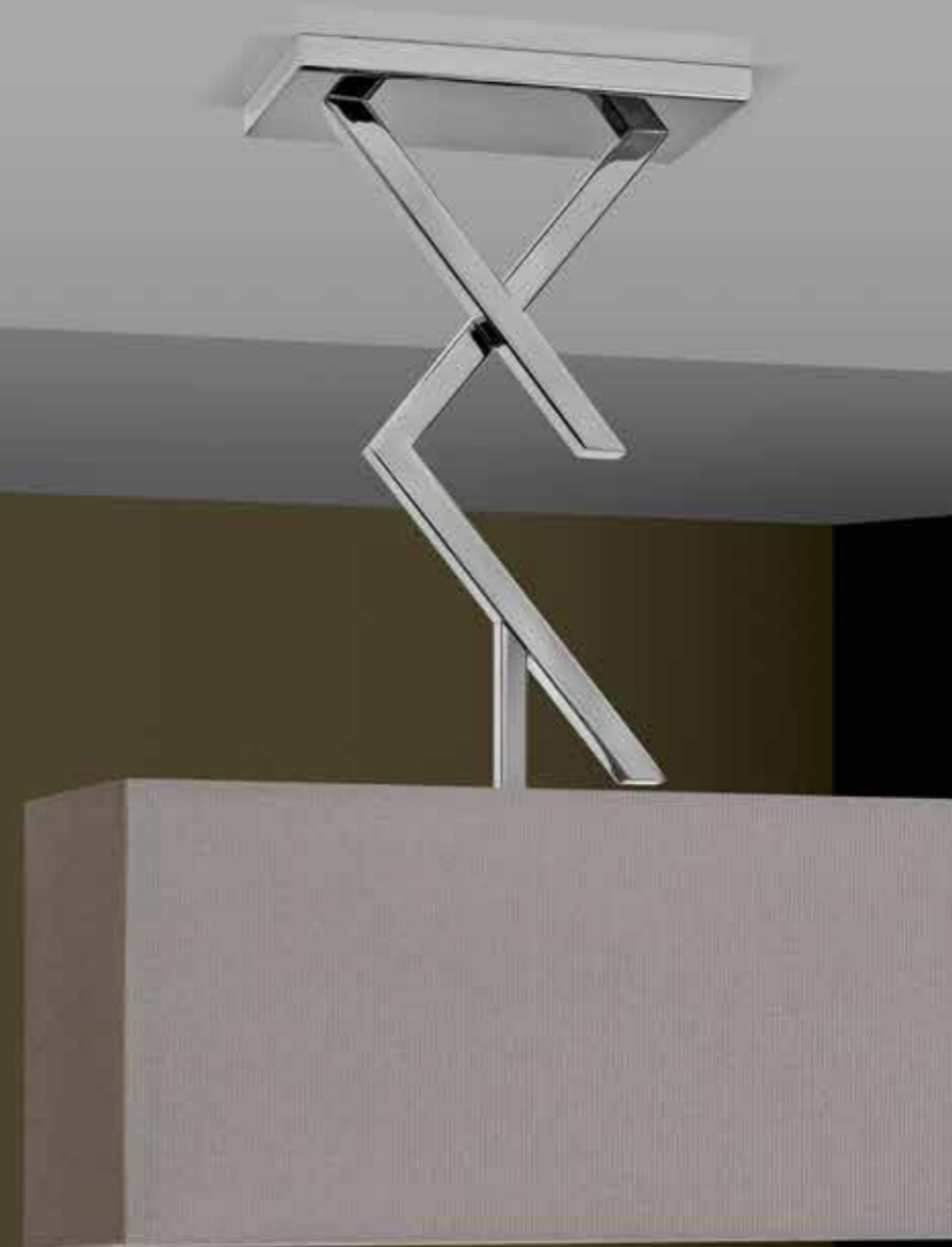
376/S CROMO COR 551 Ø 22x13 cm 50x25x50x25 cm H 47 cm H 69 cm 1 x E27 / 60W
